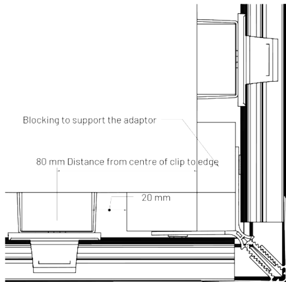
Aluminium External corner trim profile Scale 1:1
